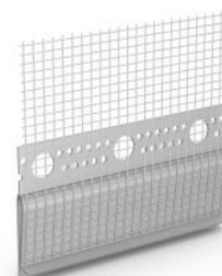
Figure 9 - Sto-Profil Jonction couvertine
